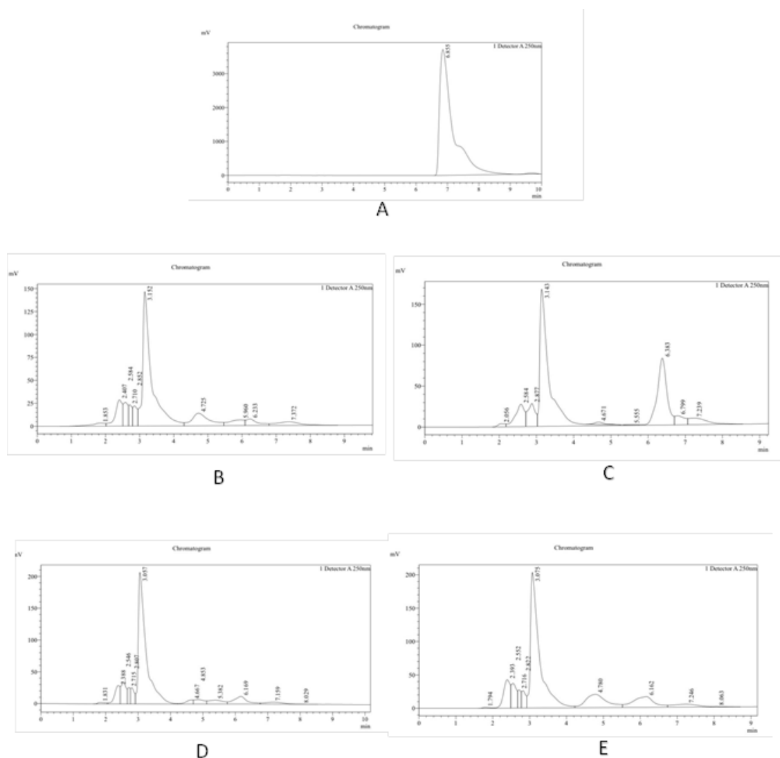
Fig. 6: Retention time of phenolic compounds isolated from stem callus extracts of P. oleracea that exposed to gamma rays at different time (0.0, 60, 120, 180) by HPLC technique.
