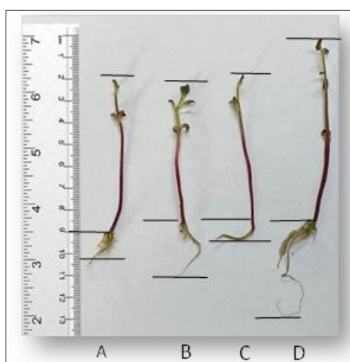
Fig. 3: Shoot and roots systems of seedlings exposed to gamma rays.
