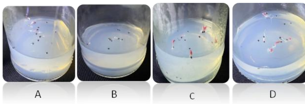
Fig. 2: Effect of gamma rays on seed germination.
